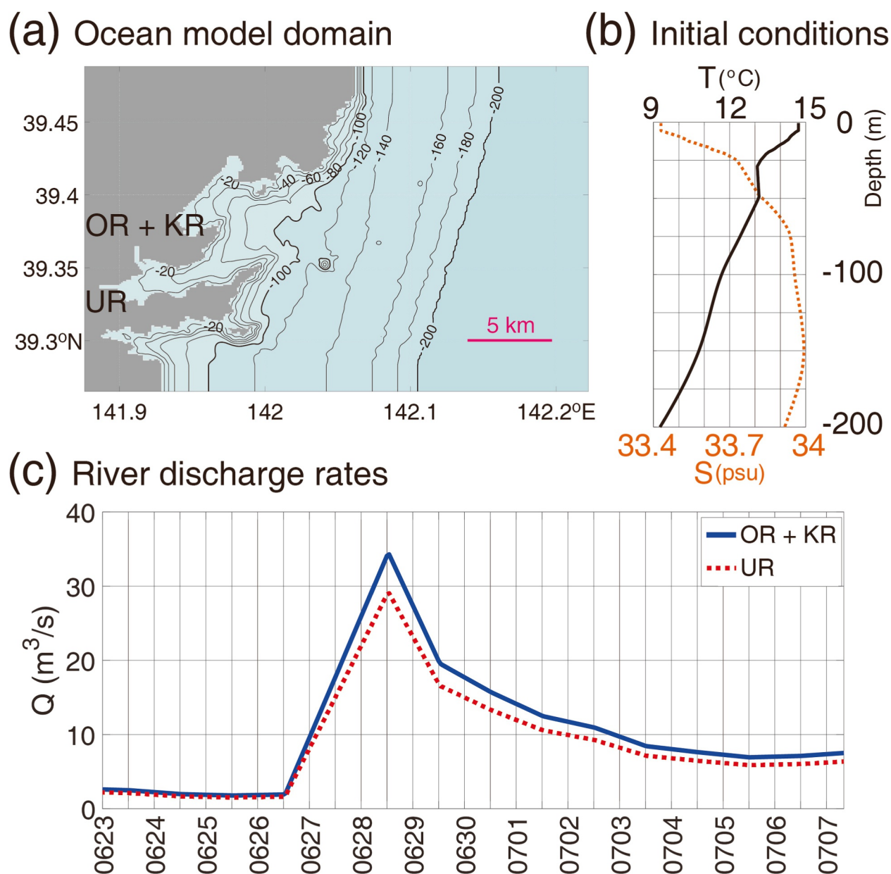
Figure 3. (a) Ocean model domain. (b) Initial conditions of temperature (T, black solid line) and salinity (S, orange dashed line). (c) River discharge rates. Freshwater fluxes were applied to the river area in (a).
