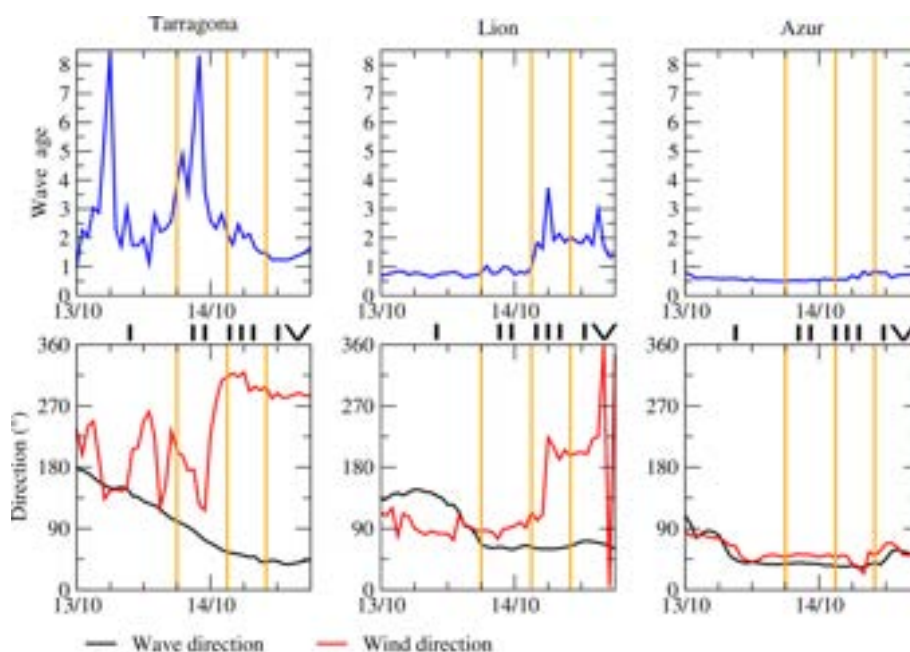
Figure 8. Evolution of the wave age (blue) and direction ( ^{\circ} ) of local wind (red) and waves (black) simulated with AWF (WY) during the 13 October run at three different moored buoys. Orange lines limit the four different phases (I, II, III and IV).
