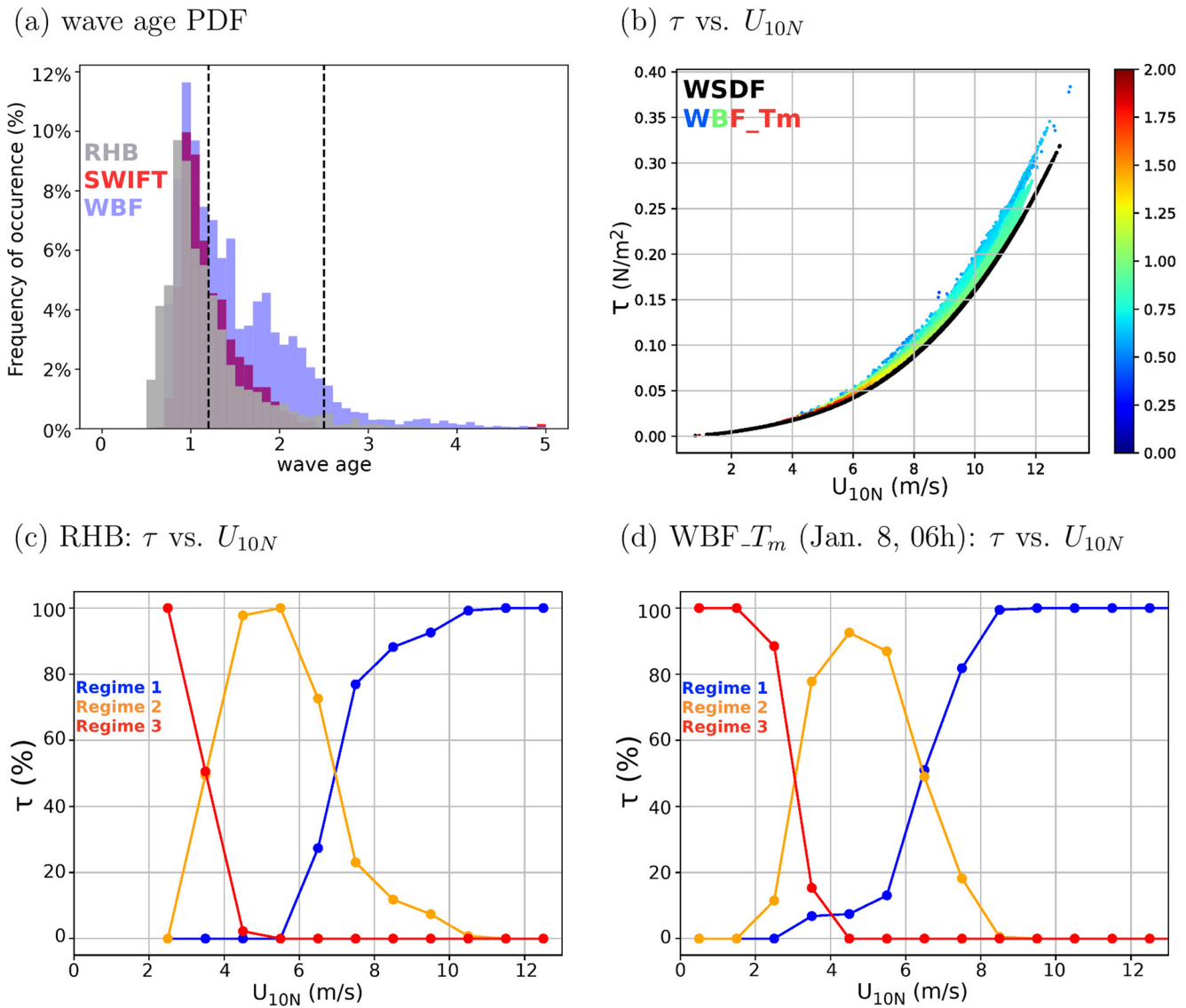
Figure 12. (a) Mean wave age distributions estimated from Ronald H. Brown (RHB) (gray), SWIFT (red), and WBF_ T_m (blue). WBF_ T_m is sampled along-track of the RHB and SWIFT. (b) Scatter plot of \tau (N m -2 ) versus U_{10N} (m s -1 ) from wind-speed-dependent formulation in black and WBF_ T_m color-coded to denote the corresponding wave age on 8 January 2020 at 0600 UTC. (c, d) As in Figures 9a and 9c, except that the wave age is defined with T_m for (c) RHB and (d) WBF_ T_m .
